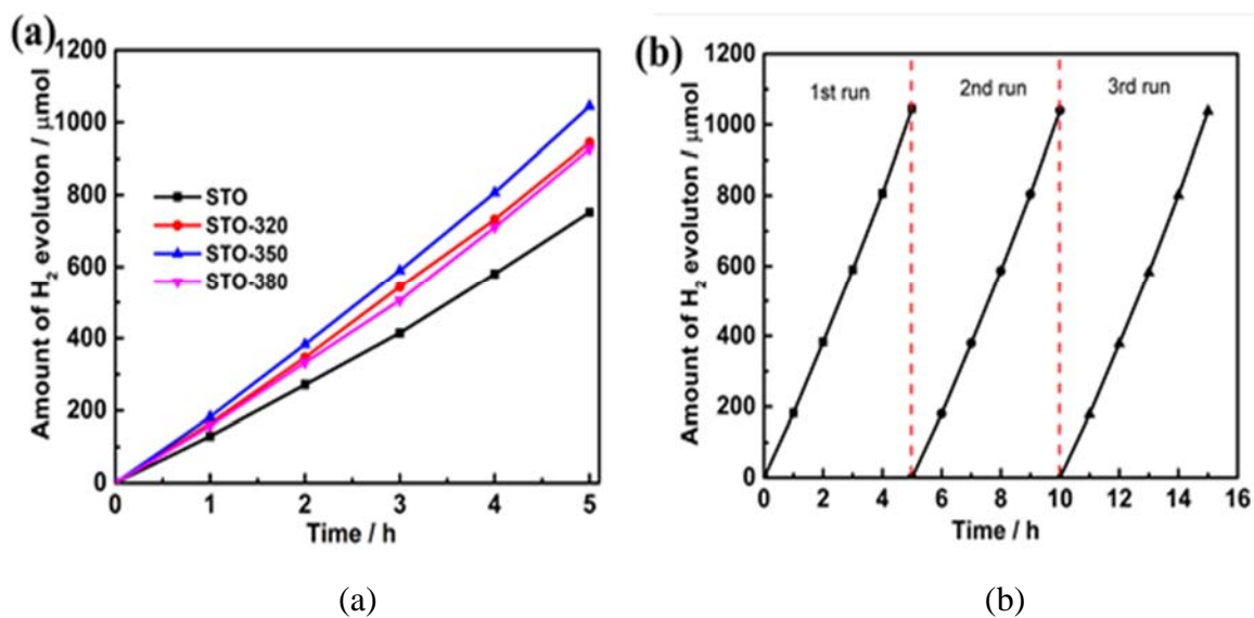
Fig. S3 Photocatalytic hydrogen production performance and stability
