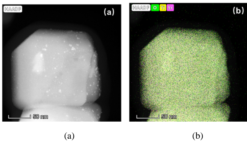
Fig. S2 All elements mapping images of STO-350
