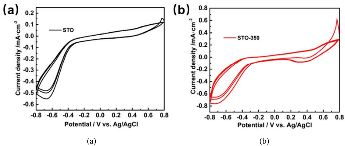
Fig. S4 CV curves in 0.1 mol/L aqueous NaSO 4
