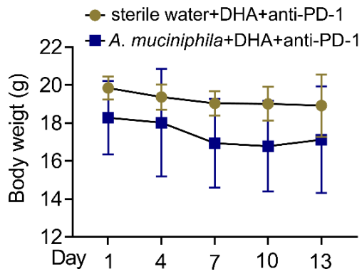
S4. The body weight of tumour-bearing mice in A. muciniphila +DHA+anti-PD-1 and sterile water+DHA+anti-PD-1 groups.
