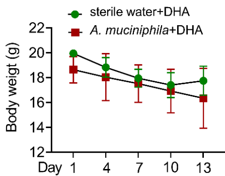
S6. The body weight of tumour-bearing mice in A. muciniphila +DHA and sterile water+DHA groups.
